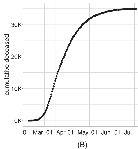
FIGURE 2 Time series of the Italian cumulative incidence indicators: cumulative positives , A and cumulative deceased , B
