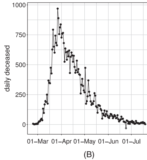
FIGURE 1 Time series of the Italian daily incidence indicators: daily positives , A and daily deceased , B
